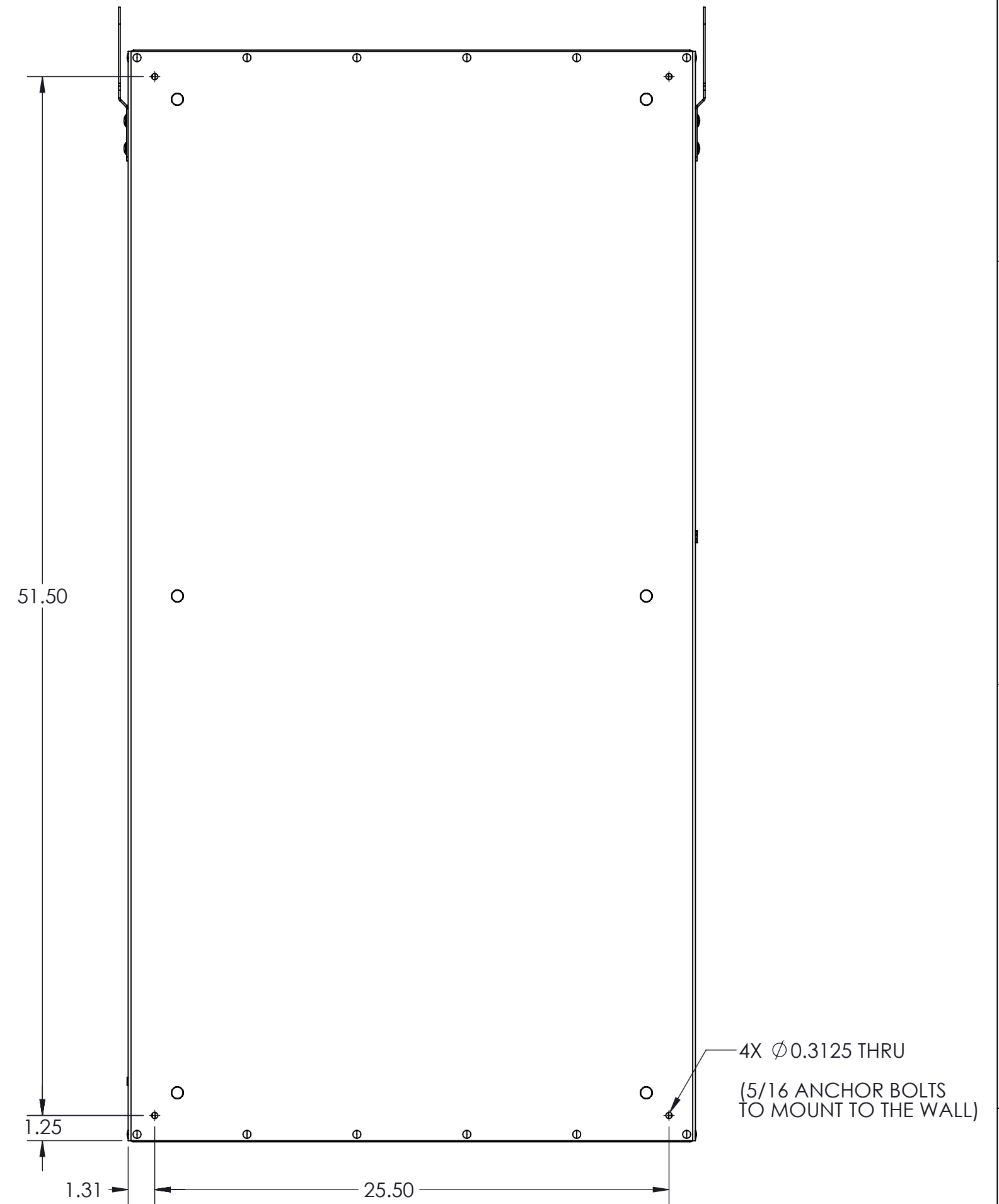
REAR VIEW
